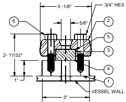
SECTION REFLEX "X-X"
