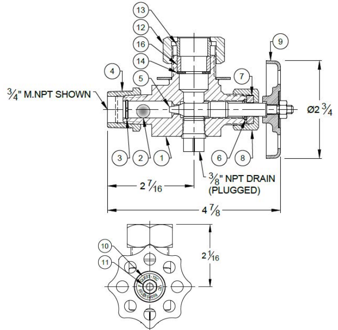
BOTTOM VALVE EXAMPLE
