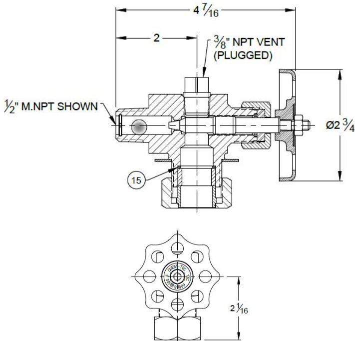
TOP VALVE EXAMPLE
