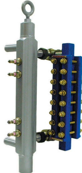
Model 501 Column with ST-1000 Level Gage
