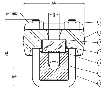
Series RM/RH Cross Section
