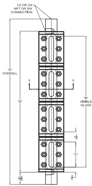
CLOSE HOOK-UP SIDE CONNECTED
