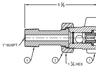
Union Male NPT
