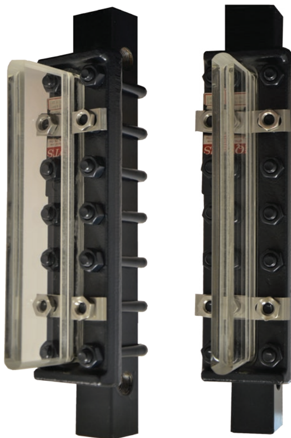
EXAMPLE: 71RL-CH-FP 4 5 / 8 " Frost-Prevention Extensions
