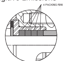
Low Emissions Packing
