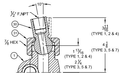
Spherical Union Female NPT [1/2" NPT only]
