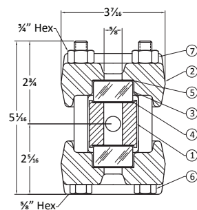
Series TM/TH Cross Section
