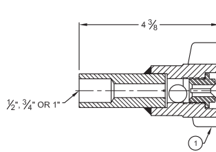
Solid Shank NPS Stub End
