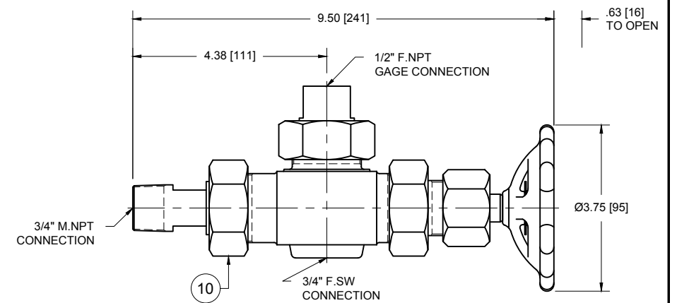
VALVE VIEW
